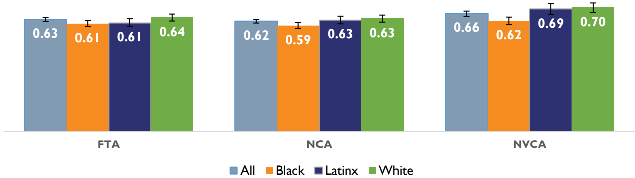
FIGURE 3. AUC-ROC Values by Race/Ethnicity
