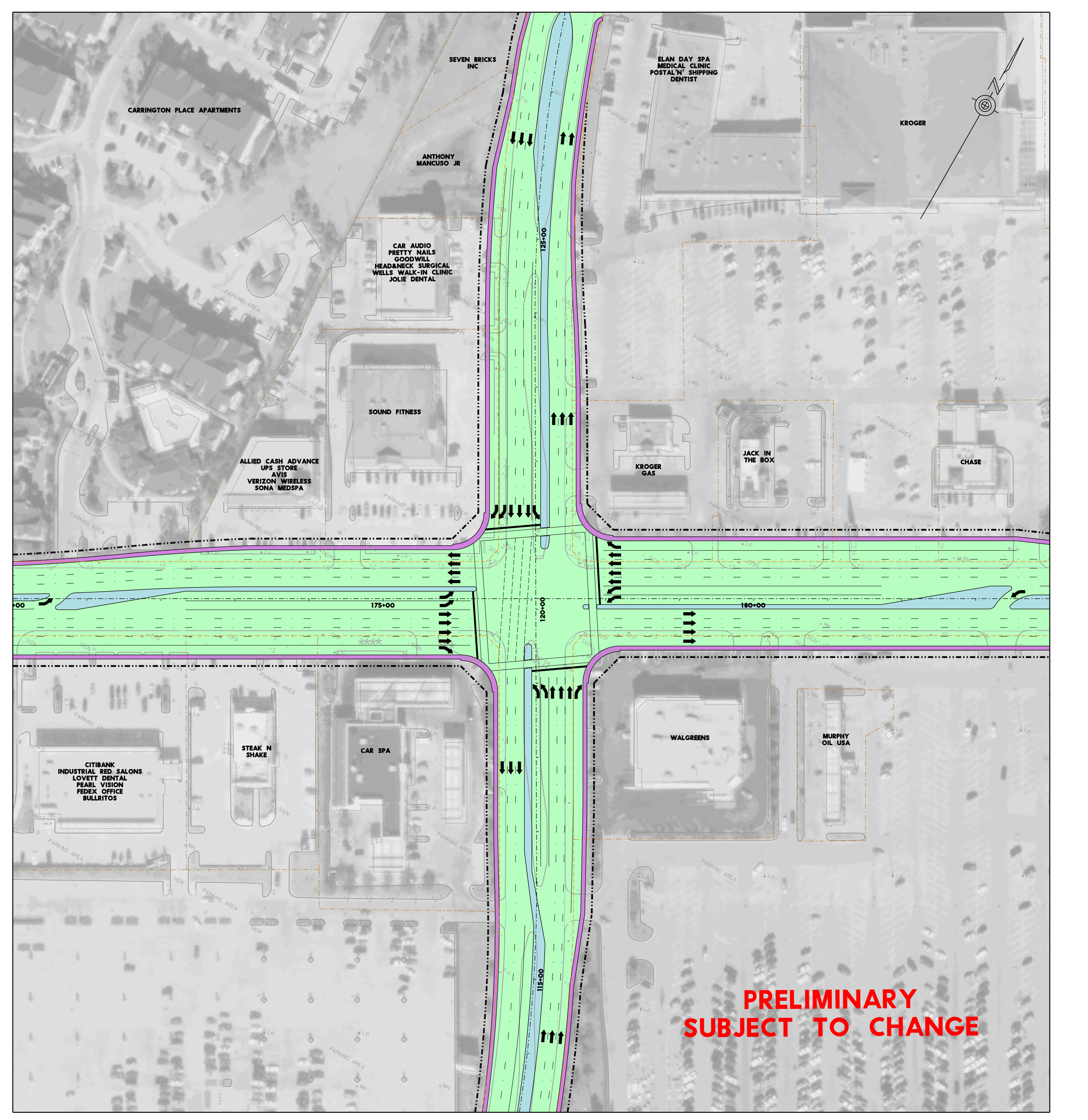
INTERSECTION DETAIL SCALE: 1" = 50'
